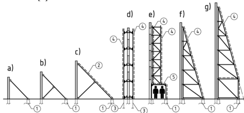
Fig. 4. Examples of design solutions of renovation bracings of angle strut-cantilevered type 1 - the temporary foundation (newly designed or used an existing one), 2 - truss or frame bracings, 3 - steel pile, 4 - truss bracing, 5 - steel portal frame
